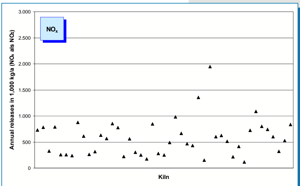
Fig. 5-4: NO x emissions (annual releases in 2007) of 45 rotary kilns
