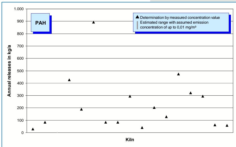
Fig. 5-16: PAH emissions (annual releases in 2007) of 17 rotary kilns. If the measurements are not secured, the releases can only be estimated. In these cases, the range of possible emissions is represented by a broken line, the upper limit of which was calculated using a concentration of 0.01 mg/m 3 .
