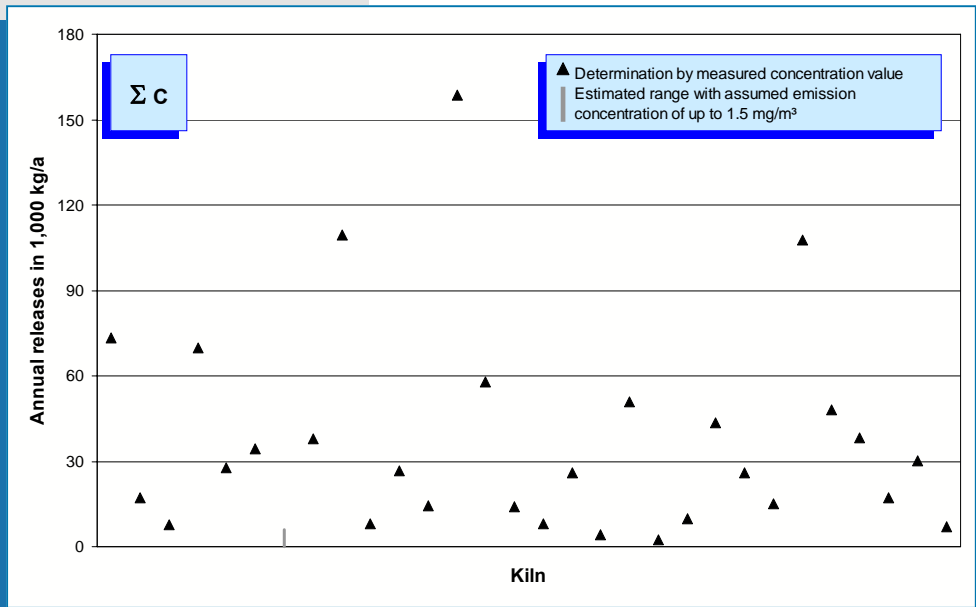
Fig. 5-10: Total organic carbon emissions (annual releases in 2007) of 30 rotary kilns. If the values measured are below the detection limit, the releases can only be estimated. In these cases, the range of possible emissions is represented by a broken line, the upper limit of which was calculated using a concentration of 1.5 mg/m 3 .
