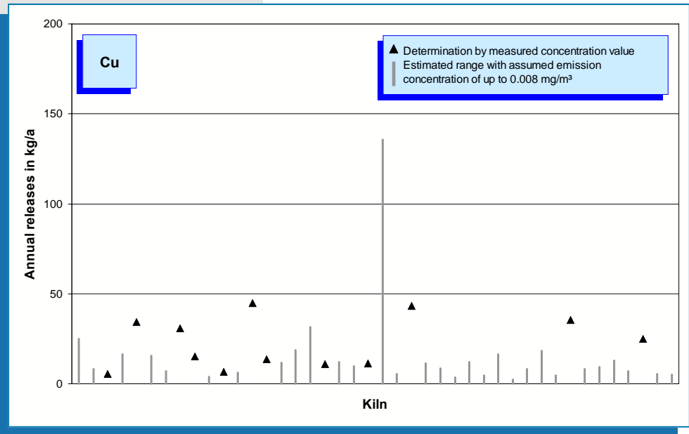
Fig. 5-42: Copper emissions (annual releases in 2007) of 42 rotary kilns. If the values measured are below the detection limit, the releases can only be estimated. In these cases, the range of possible emissions is represented by a broken line, the upper limit of which was calculated using a concentration of 0.008 mg/m 3 .
