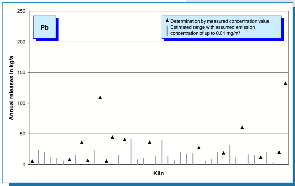
Fig. 5-36: Lead emissions (annual releases in 2007) of 42 rotary kilns.
