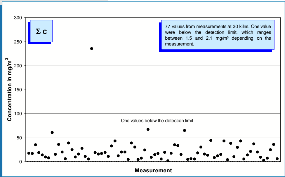
Fig. 5-9: Total organic carbon concentration values (year 2007) measured in the clean gas of 30 rotary kilns.
