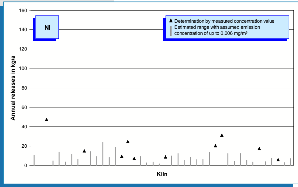
Fig. 5-46: Nickel emissions (annual releases in 2007) of 42 rotary kilns. If the values measured are below the detection limit, the releases can only be estimated. In these cases, the range of possible emissions is represented by a broken line, the upper limit of which was calculated using a concentration of 0.006 mg/m 3 .
