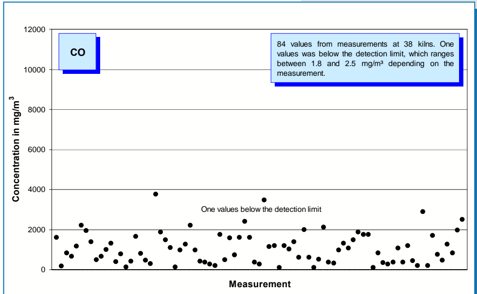
Fig. 5-7: CO concentration values (year 2007) measured in the clean gas of 38 rotary kilns.
