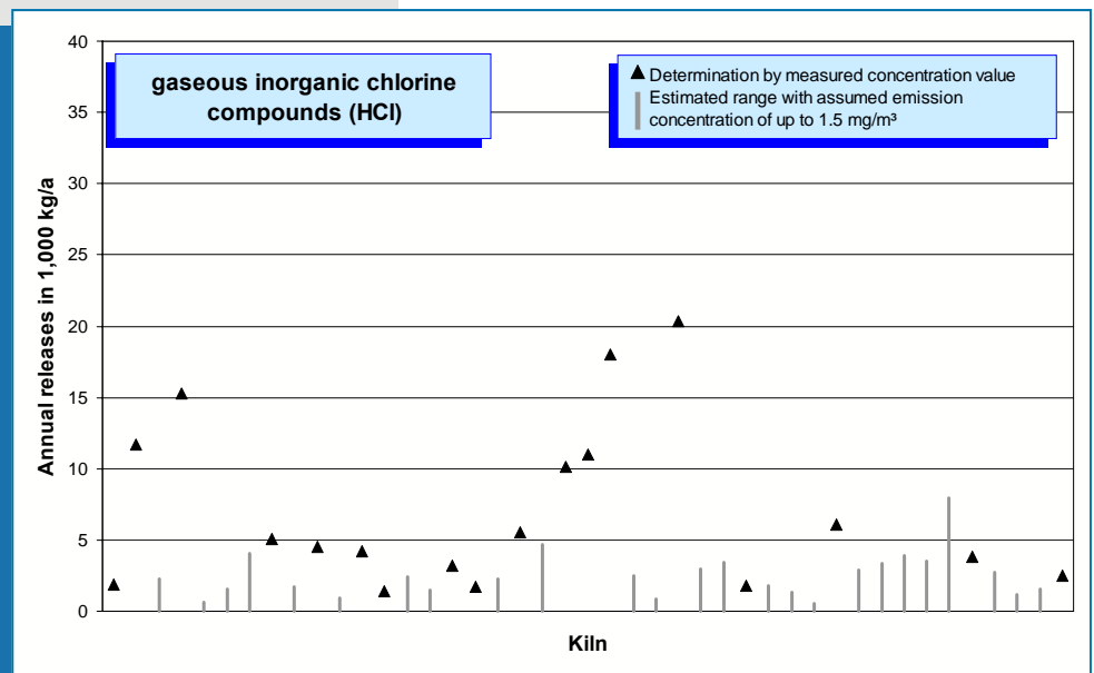
Fig. 5-22: HCl emissions (annual releases in 2007) of 43 rotary kilns.
