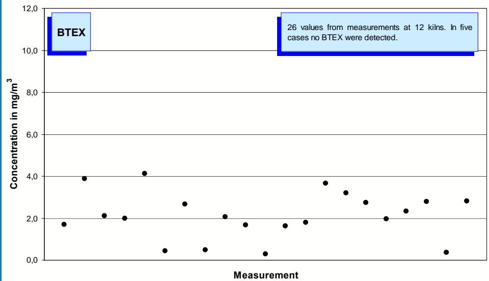
Fig. 5-17: BTEX concentration values (year 2007) measured in the clean gas of 12 rotary kilns. In five cases no BTEX were detected.
