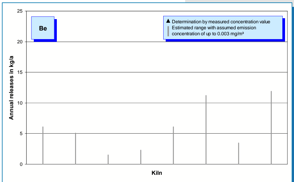
Fig. 5-52: Beryllium emissions (annual releases in 2007) of eight rotary kilns.
