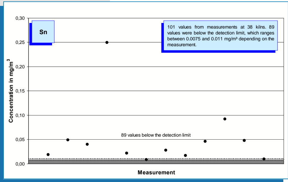
Fig. 5-49: Tin concentration values (year 2007) measured in the clean gas of 38 rotary kilns.
