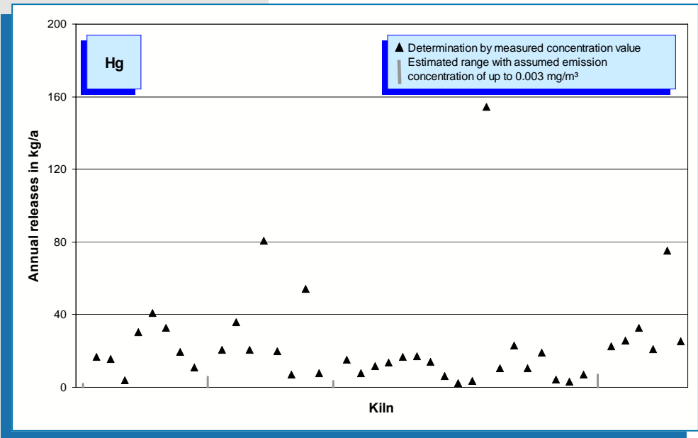
Fig. 5-30: Mercury emissions (annual releases in 2007) of 44 rotary kilns. If the values measured are below the detection limit, the releases can only be estimated. In these cases, the range of possible emissions is represented by a broken line, the upper limit of which was calculated using a concentration of 0.003 mg/m 3 .
