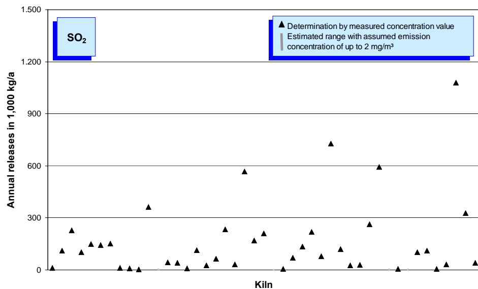
Fig. 5-6: SO 2 emissions (annual releases in 2007) of 45 rotary kilns.
