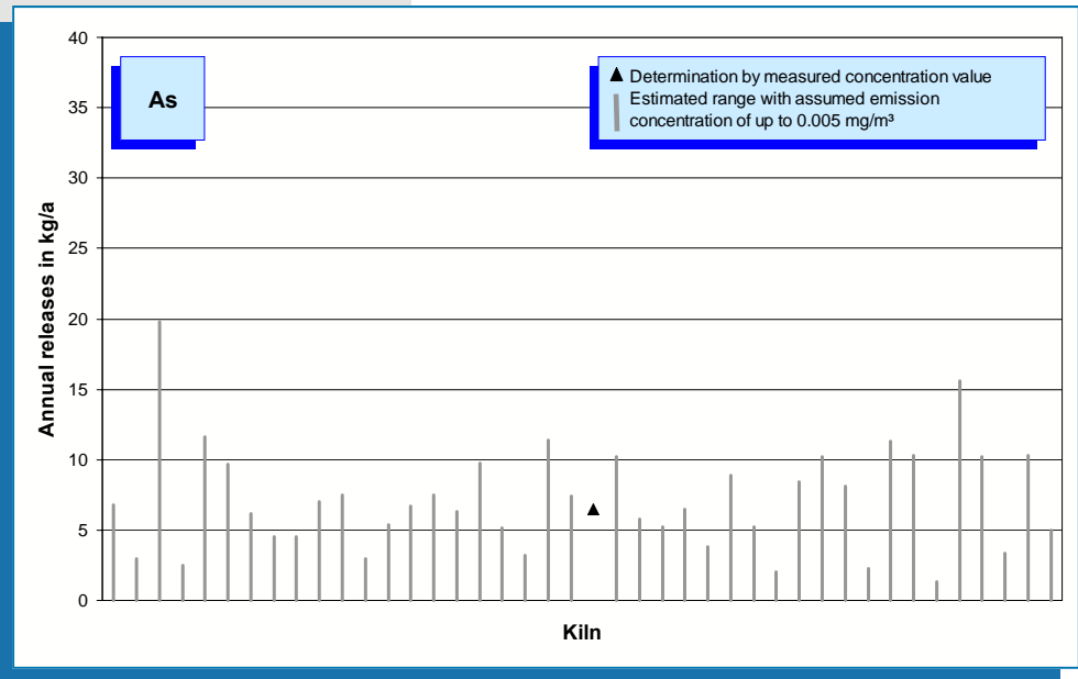
Fig. 5-34: Arsenic emissions (annual releases in 2007) of 42 rotary kilns. If the values measured are below the detection limit, the releases can only be estimated. In these cases, the range of possible emissions is represented by a broken line, the upper limit of which was calculated using a concentration of 0.005 mg/m 3 .
