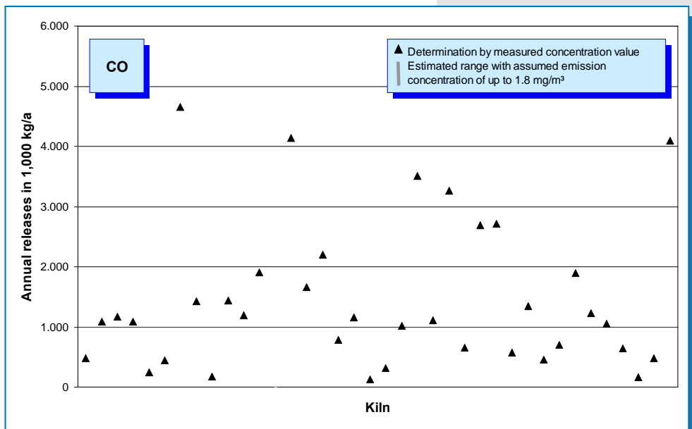
Fig. 5-8: CO emissions (annual releases in 2007) of 38 rotary kilns.
