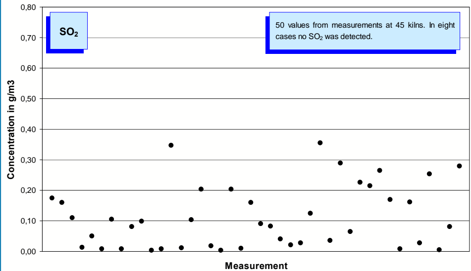
Fig. 5-5: Average SO 2 concentrations (year 2007) in the clean gas of 45 rotary kilns.
