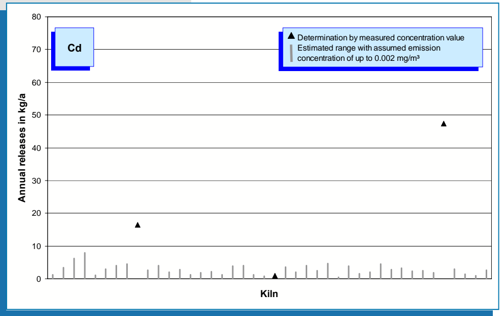
Fig. 5-26: Cadmium emissions (annual releases in 2007) of 42 rotary kilns. If the values measured are below the detection limit, the releases can only be estimated. In these cases, the range of possible emissions is represented by a broken line, the upper limit of which was calculated using a concentration of 0.002 mg/m 3 .
