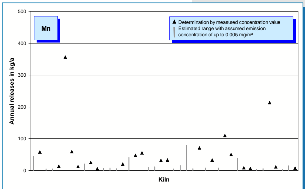
Fig. 5-44: Manganese emissions (annual releases in 2007) of 42 rotary kilns.
