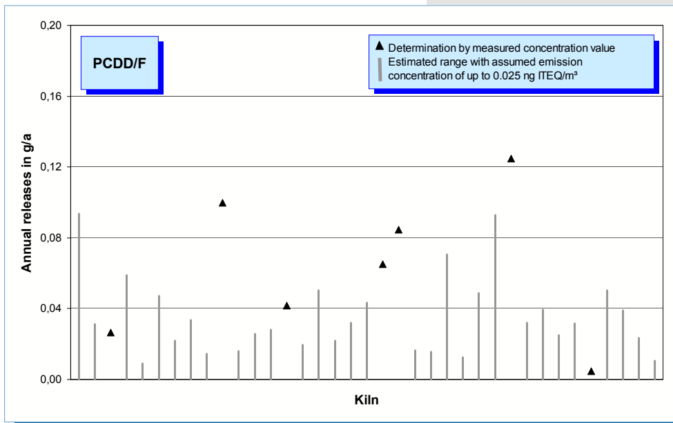
Fig. 5-12: Dioxin and furan emissions (annual releases in 2005) of 37 rotary kilns.
