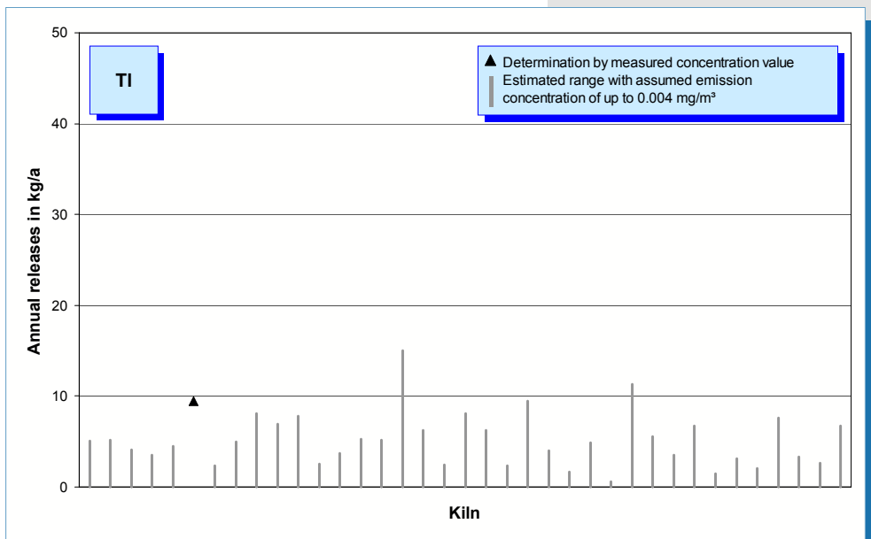
Fig. 5-28: Thallium emissions (annual releases in 2005) of 37 rotary kilns.
