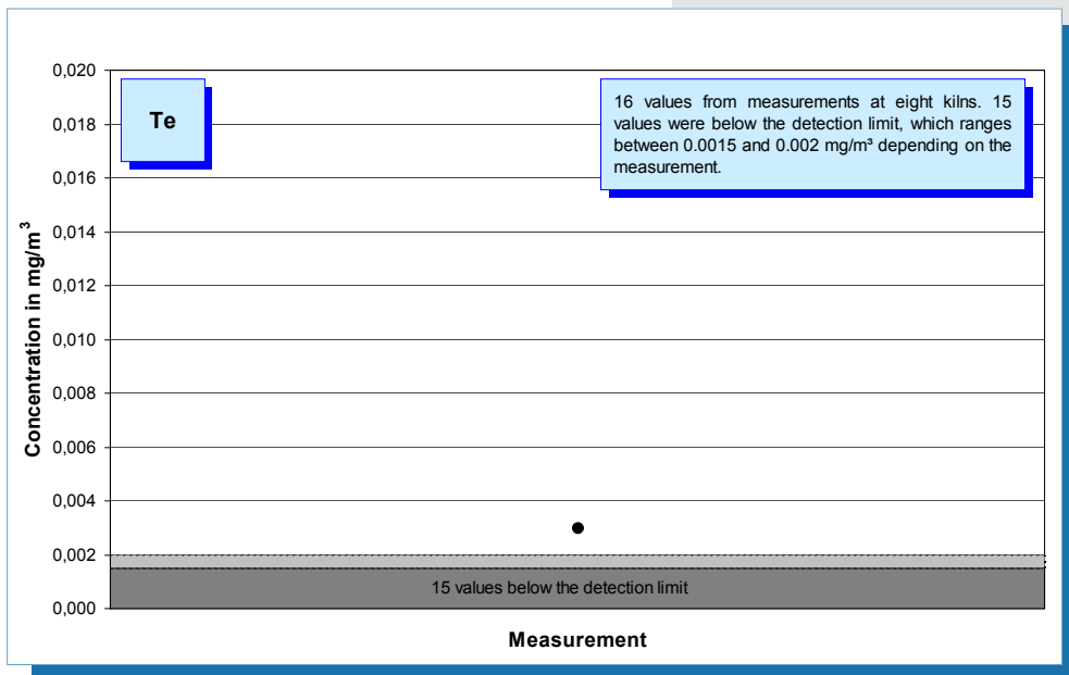
Fig. 5-55: Tellurium concentration values (year 2005) measured in the clean gas of eight rotary kilns.
