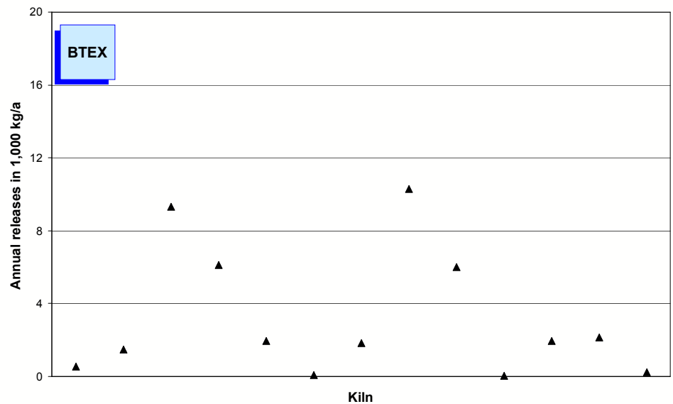
Fig. 5-18: BTEX emissions (annual releases in 2005) of 13 rotary kilns.
