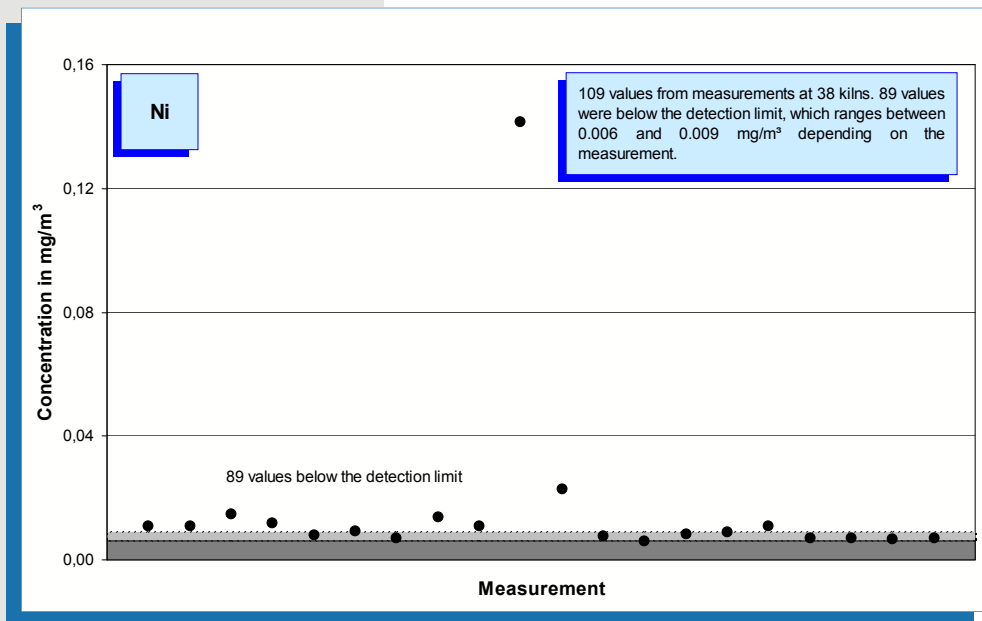
Fig. 5-45: Nickel concentration values (year 2005) measured in the clean gas of 38 rotary kilns.
