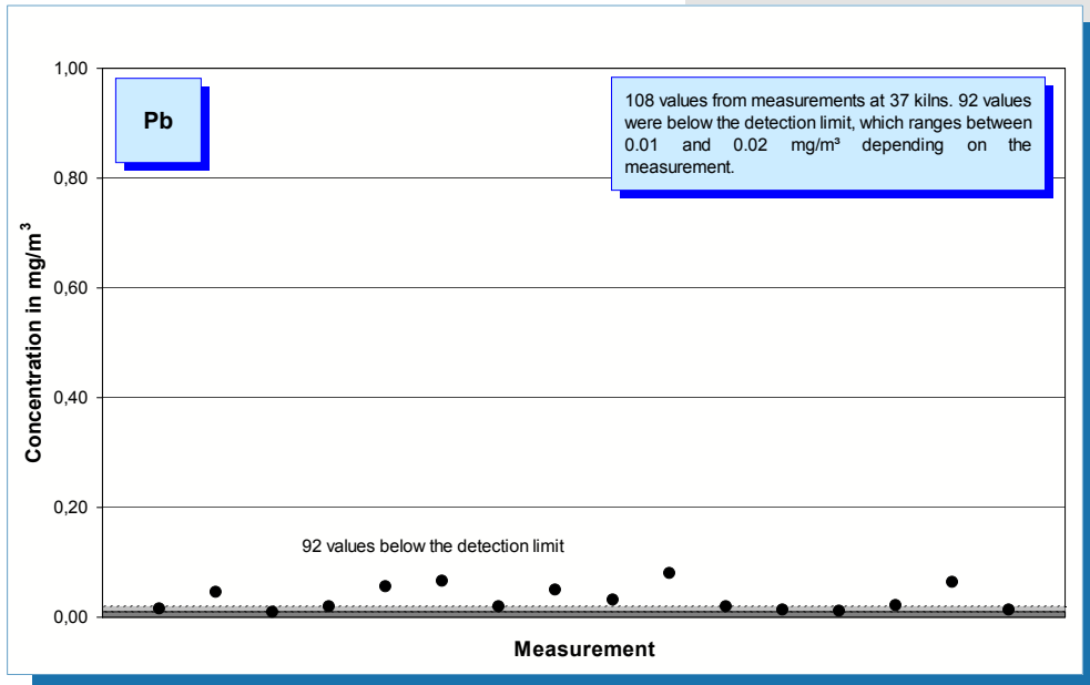
Fig. 5-35: Lead concentration values (year 2005) measured in the clean gas of 37 rotary kilns.
