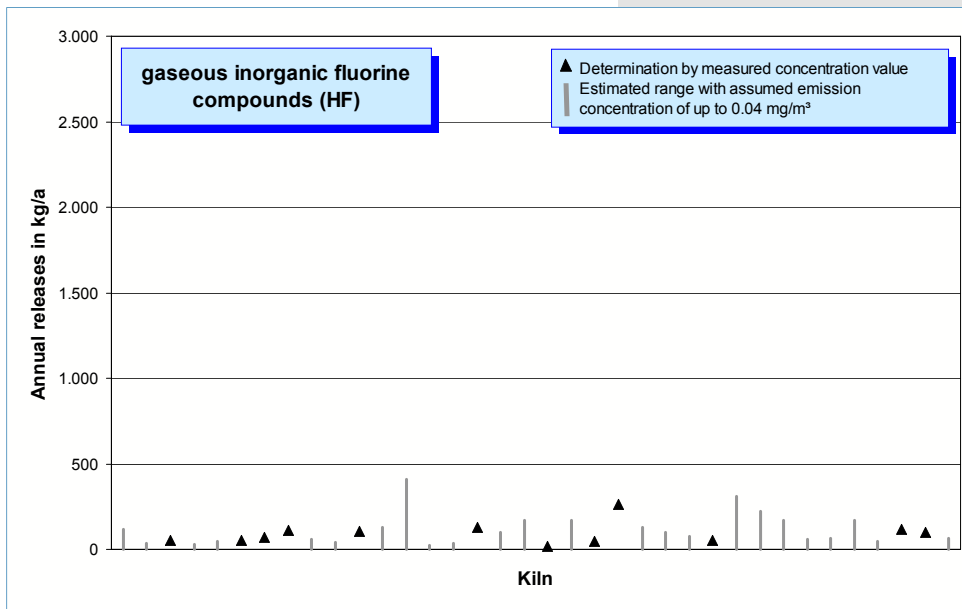
Fig. 5-24: HF emissions (annual releases in 2005) of 36 rotary kilns.
