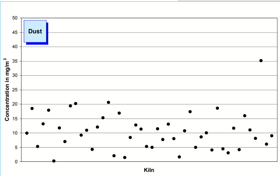
Fig. 5-1: Average (year 2005) dust concentrations in the clean gas of 46 rotary kilns
