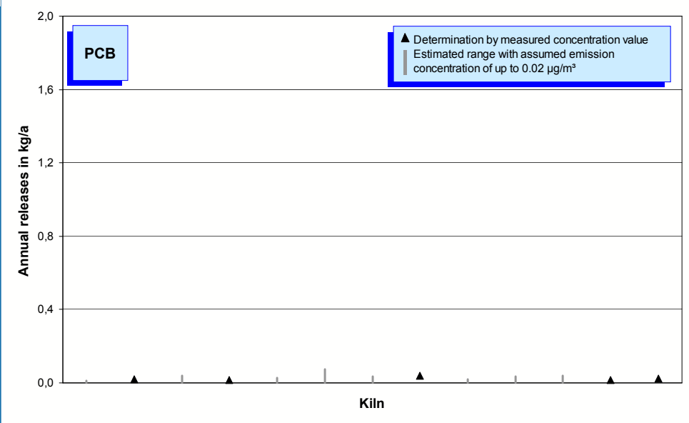
Fig. 5-14: PCB emissions (annual releases in 2005) of 13 rotary kilns.
