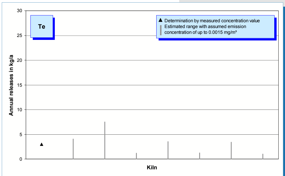
Fig. 5-56: Tellurium emissions (annual releases in 2005) of eight rotary kilns.
