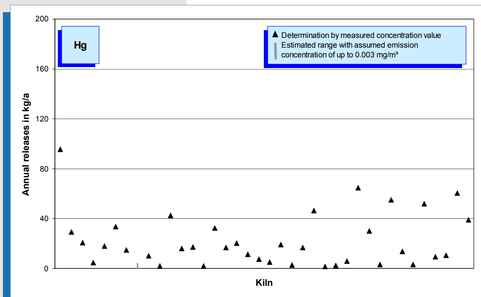
Fig. 5-30: Mercury emissions (annual releases in 2005) of 38 rotary kilns.
