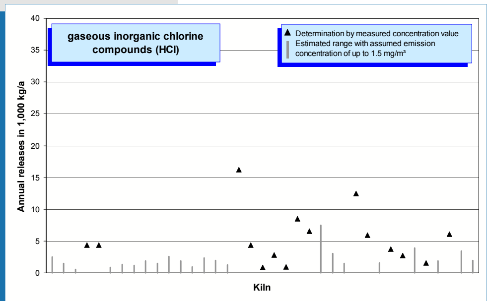
Fig. 5-22: HCl emissions (annual releases in 2005) of 37 rotary kilns.
