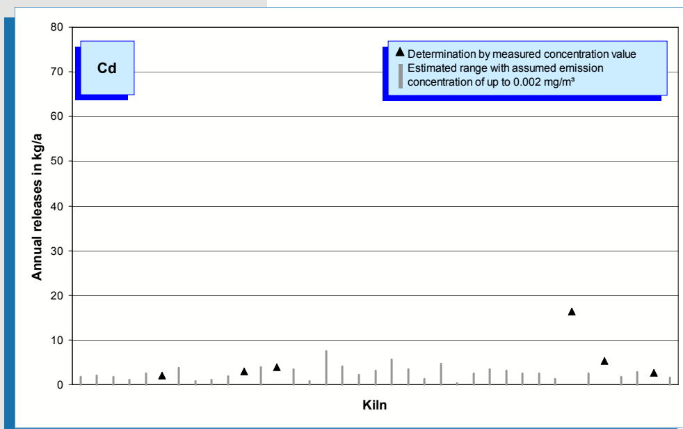
Fig. 5-26: Cadmium emissions (annual releases in 2005) of 37 rotary kilns.
