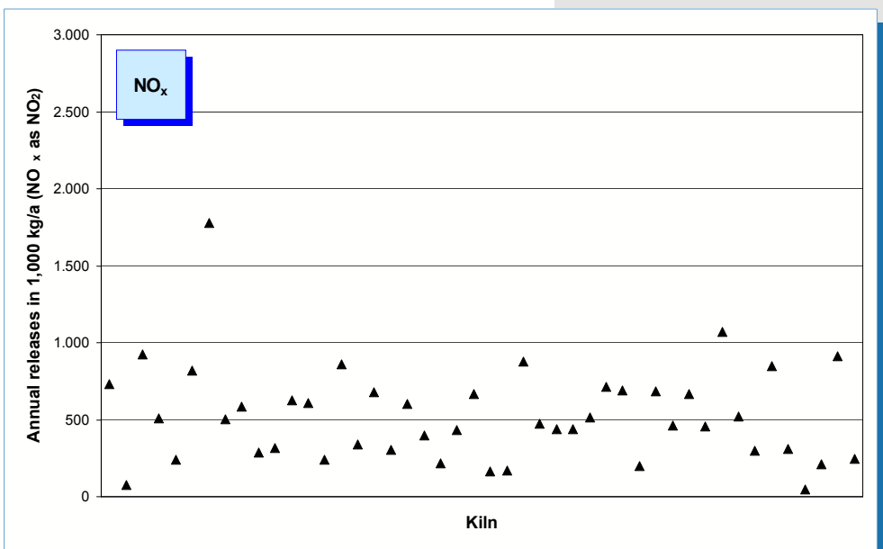
Fig. 5-4: NO x emissions (annual releases in 2005) of 46 rotary kilns
