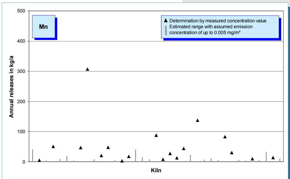
Fig. 5-44: Manganese emissions (annual releases in 2005) of 37 rotary kilns.
