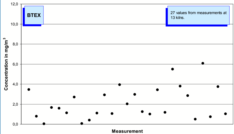
Fig. 5-17: BTEX concentration values (year 2005) measured in the clean gas of 13 rotary kilns. No detection limit can be deduced from the standard. Below 0.013 mg/m 3 the measuring methods currently used do not provide secured emission concentrations.
