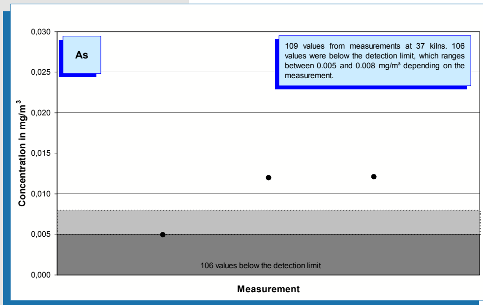
Fig. 5-33: Arsenic concentration values (year 2005) measured in the clean gas of 37 rotary kilns.
