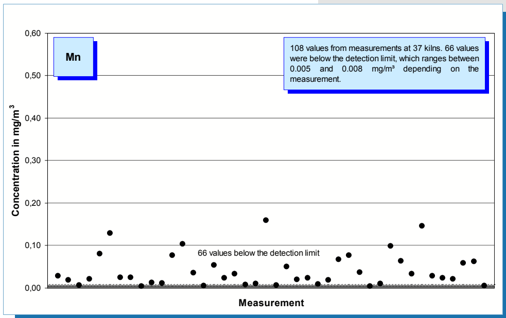
Fig. 5-43: Manganese concentration values (year 2005) measured in the clean gas of 37 rotary kilns.
