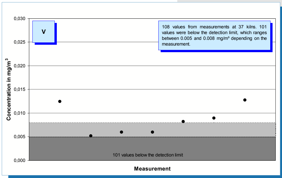
Fig. 5-47: Vanadium concentration values (year 2005) measured in the clean gas of 37 rotary kilns.
