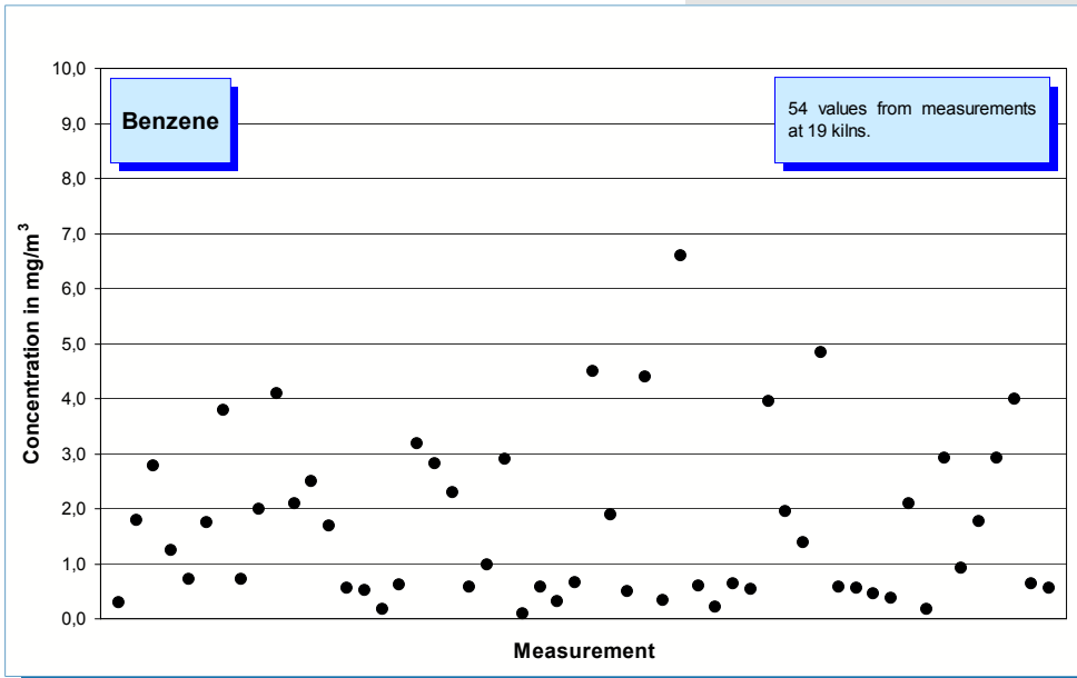
Fig. 5-19: Benzene concentration values (year 2005) measured in the clean gas of 19 rotary kilns. No detection limit can be deduced from the standard. Below 0.013 mg/m 3 the measuring methods currently used do not provide secured emission concentrations.
