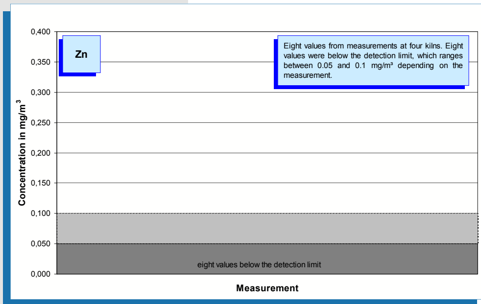
Fig. 5-57: Zinc concentration values (year 2005) measured in the clean gas of four rotary kilns.
