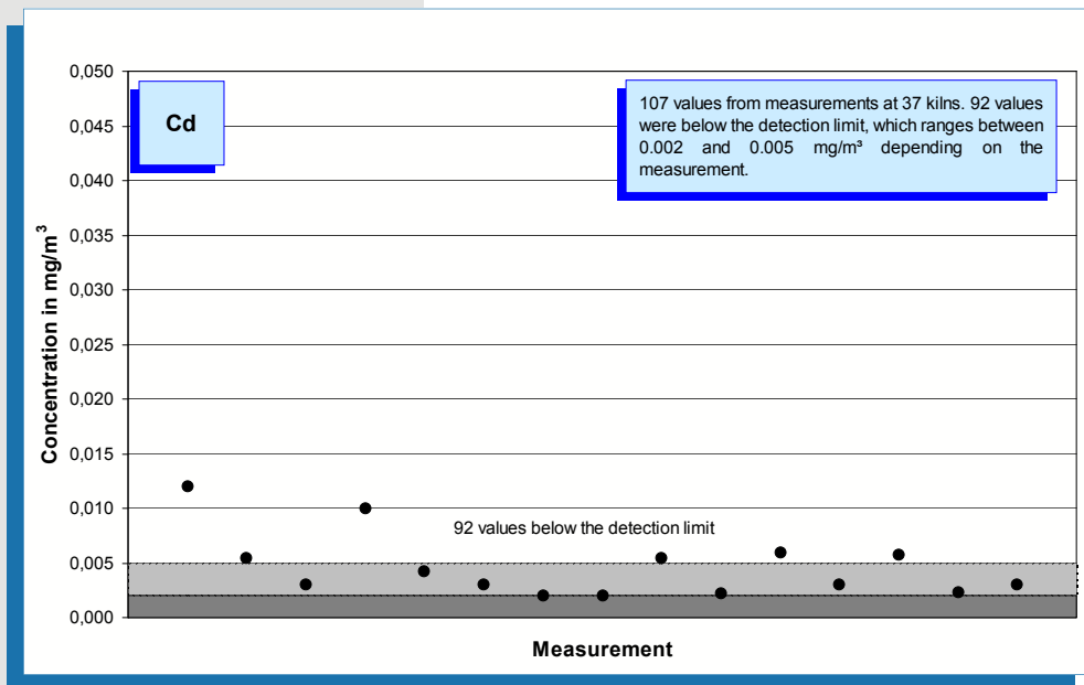
Fig. 5-25: Cadmium concentration values (year 2005) measured in the clean gas of 37 rotary kilns.
