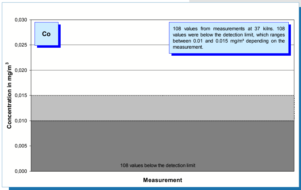
Fig. 5-39: Cobalt concentration values (year 2005) measured in the clean gas of 37 rotary kilns.
