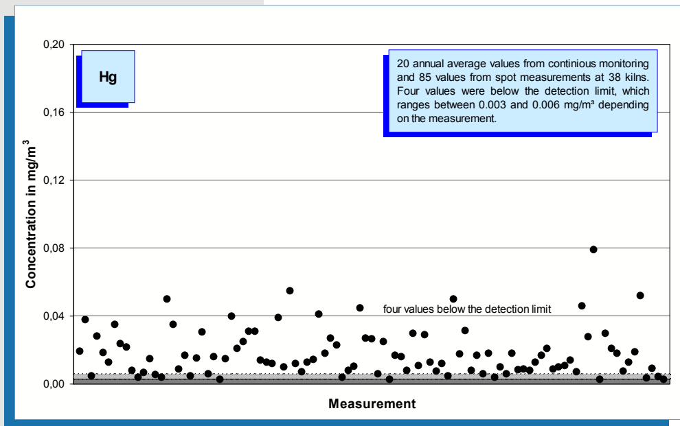
Fig. 5-29: Mercury concentration values (year 2005) measured in the clean gas of 38 rotary kilns.
