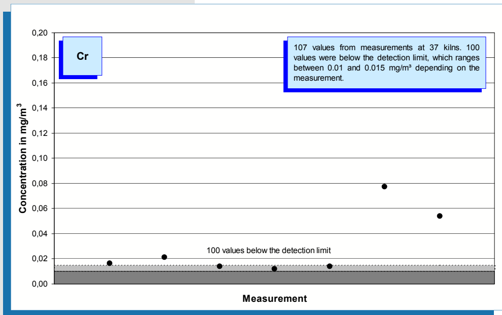
Fig. 5-37: Chromium concentration values (year 2005) measured in the clean gas of 37 rotary kilns.
