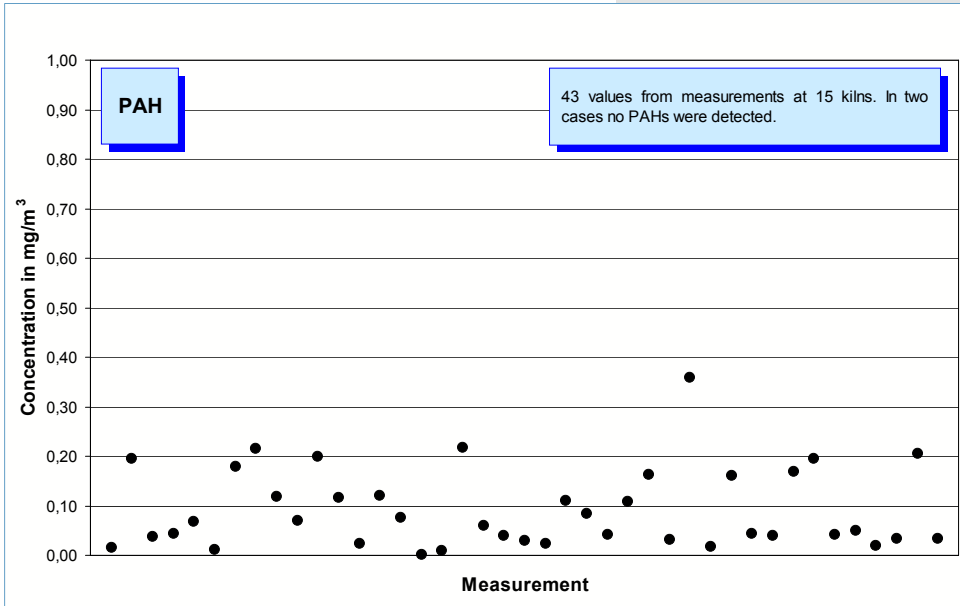
Fig. 5-15: Polycyclic aromatic hydrocarbon (PAH according to EPA 610) concentration values (year 2005) measured in the clean gas of 15 rotary kilns. In two cases no PAHs were detected.
