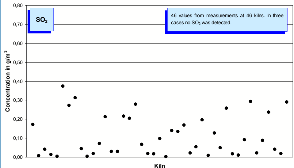
Fig. 5-5: Average SO 2 concentrations (year 2005) in the clean gas of 46 rotary kilns.
