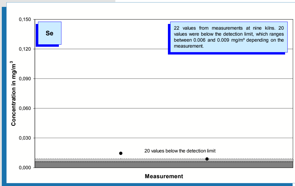
Fig. 5-53: Selenium concentration values (year 2005) measured in the clean gas of nine rotary kilns.
