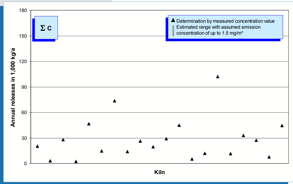
Fig. 5-10: Total organic carbon emissions (annual releases in 2005) of 20 rotary kilns. If the values measured are below the detection limit, the releases can only be estimated. In these cases, the range of possible emissions is represented by a broken line, the upper limit of which was calculated using a concentration of 1.5 mg/m 3 .
