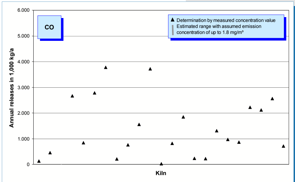
Fig. 5-8: CO emissions (annual releases in 2005) of 23 rotary kilns.
