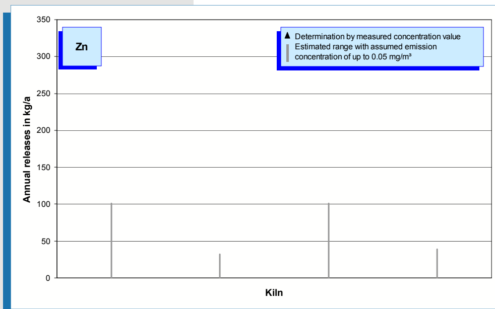
Fig. 5-58: Zinc emissions (annual releases in 2005) of four rotary kilns.
