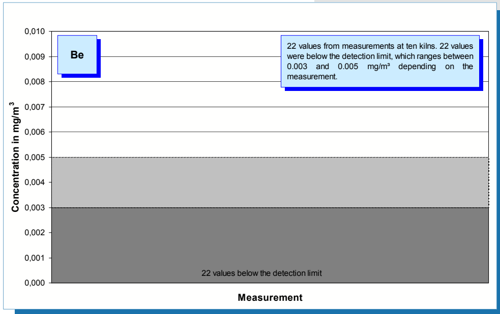
Fig. 5-51: Beryllium concentration values (year 2005) measured in the clean gas of ten rotary kilns.
