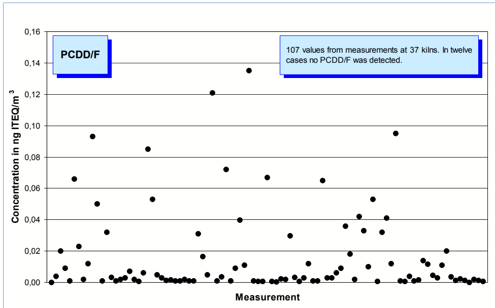
Fig. 5-11: Dioxin and furan (PCDD/F) concentration values (year 2005) measured in the clean gas of 37 rotary kilns. In twelve cases no PCDD/F was detected. Note: No detection limit can be deduced from the standard. To evaluate the measurement results, inter-laboratory variation of the method (comparison between different laboratories) can be referred to. Pursuant to DIN EN 1948 it amounts to \pm 0.05 ng ITEQ/m 3 . (ITEQ: international toxicity equivalent)
