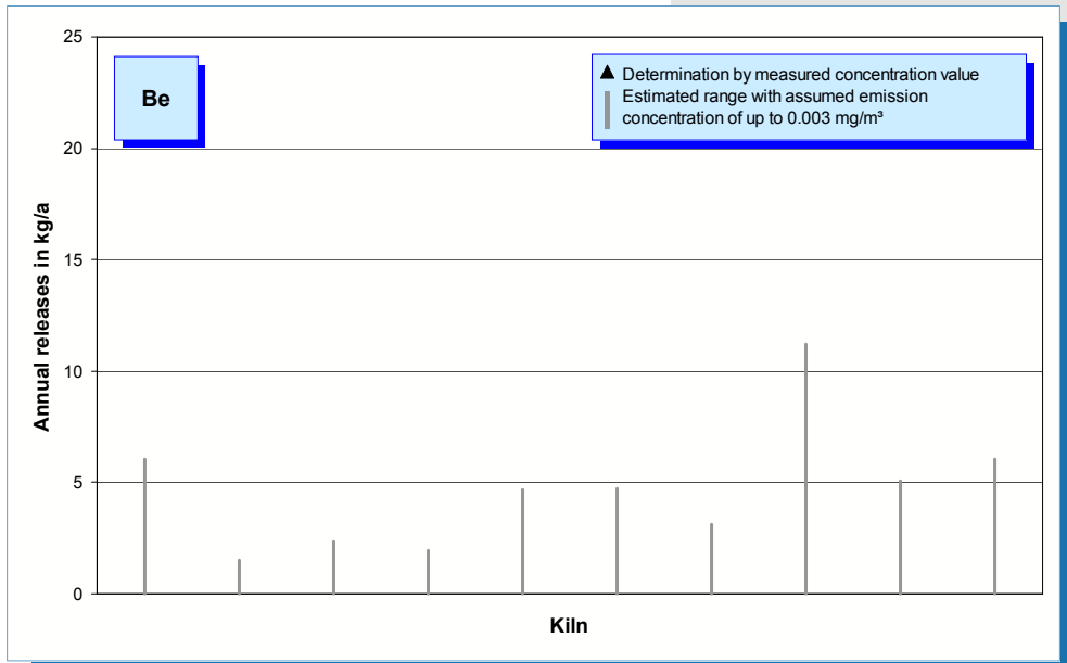
Fig. 5-52: Beryllium emissions (annual releases in 2005) of ten rotary kilns.
