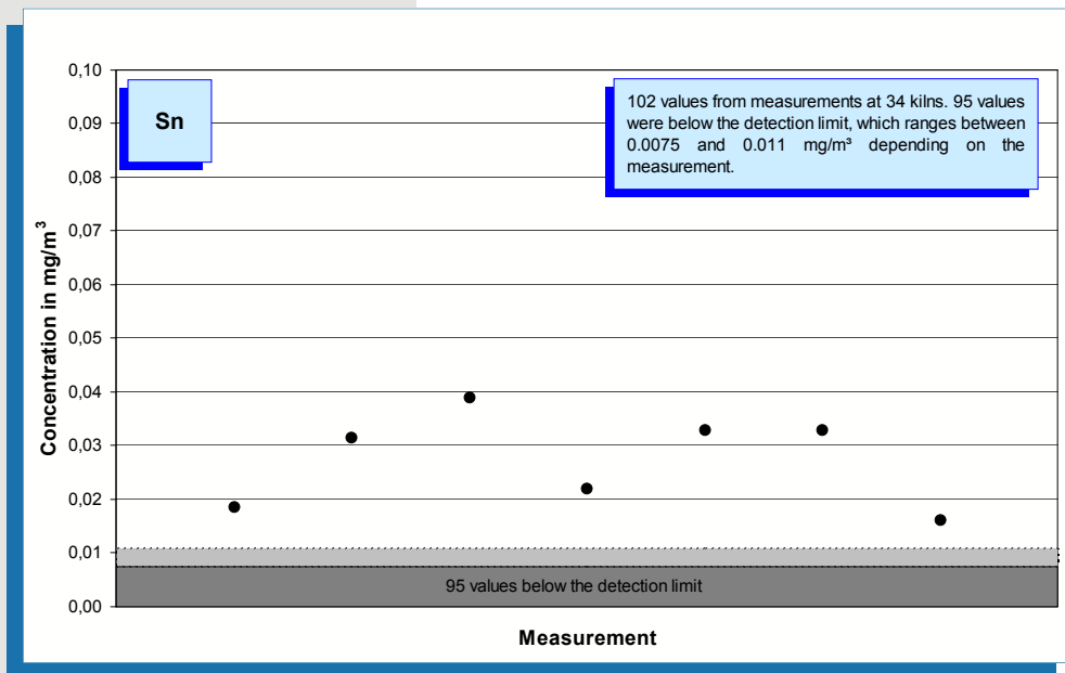
Fig. 5-49: Tin concentration values (year 2005) measured in the clean gas of 34 rotary kilns.
