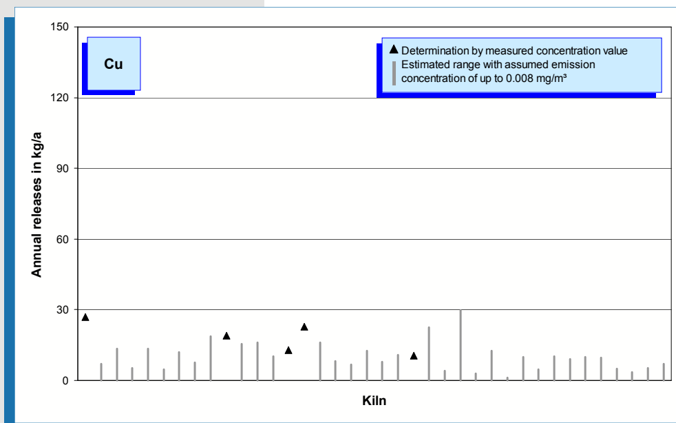
Fig. 5-42: Copper emissions (annual releases in 2005) of 38 rotary kilns.
