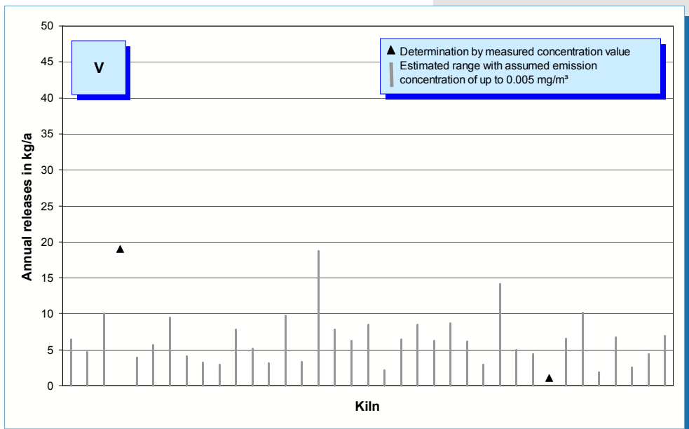
Fig. 5-48: Vanadium emissions (annual releases in 2005) of 37 rotary kilns.
