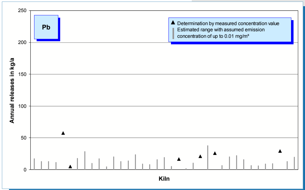
Fig. 5-36: Lead emissions (annual releases in 2005) of 37 rotary kilns.
