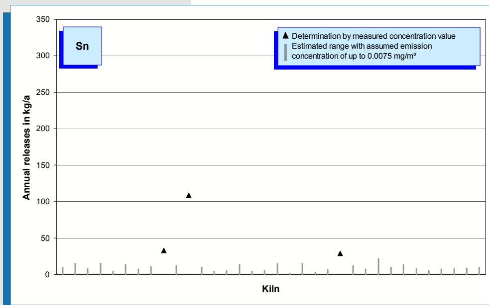
Fig. 5-50: Tin emissions (annual releases in 2005) of 34 rotary kilns.
