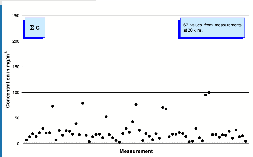
Fig. 5-9: Total organic carbon concentration values (year 2005) measured in the clean gas of 20 rotary kilns.
