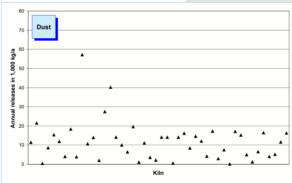
Fig. 5-2: Dust emissions (annual releases in 2005) of 46 rotary kilns
