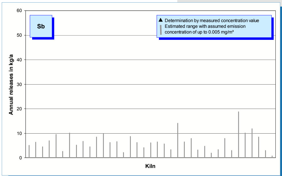
Fig. 5-32: Antimony emissions (annual releases in 2005) of 37 rotary kilns.
