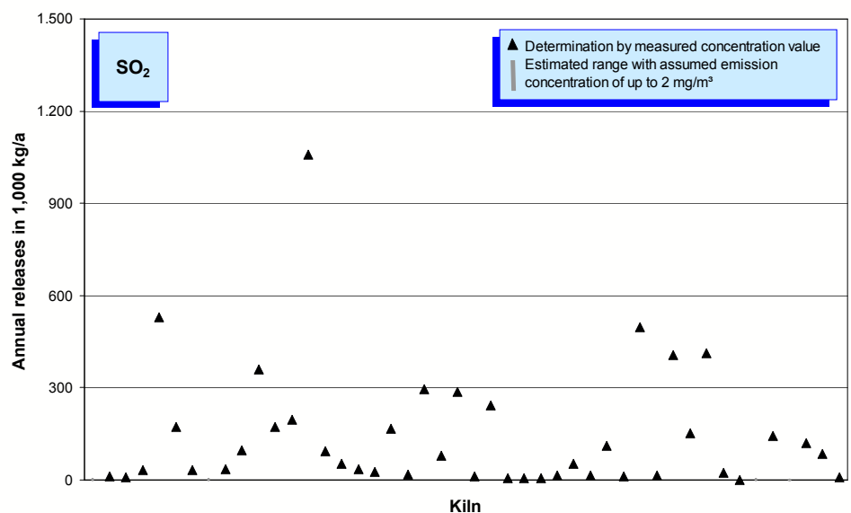
Fig. 5-6: SO 2 emissions (annual releases in 2005) of 46 rotary kilns.
