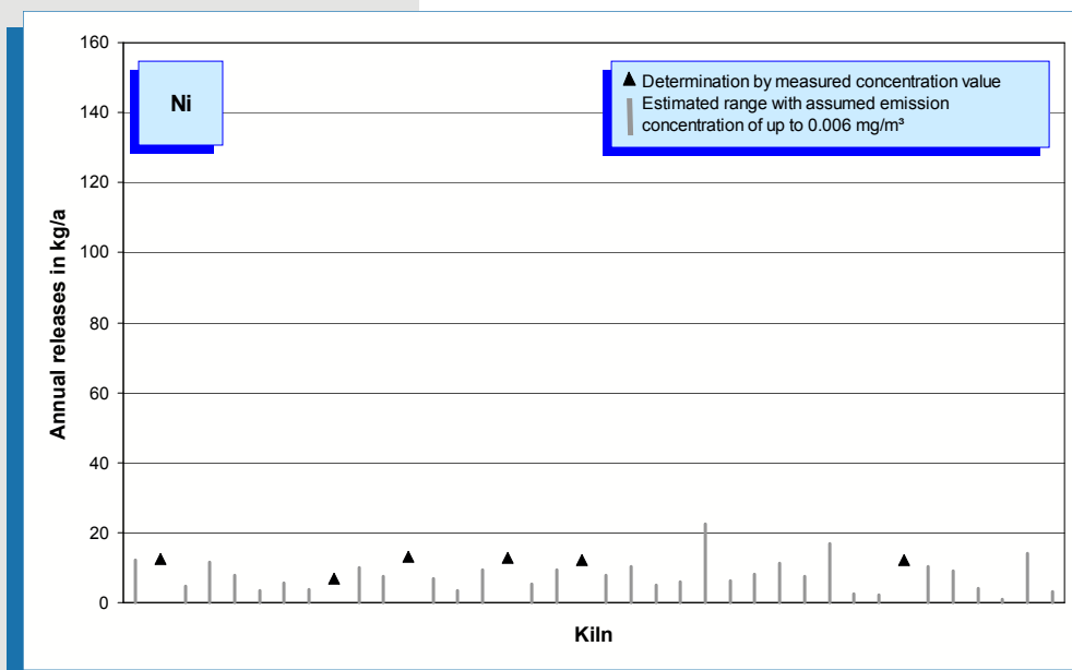
Fig. 5-46: Nickel emissions (annual releases in 2005) of 38 rotary kilns.
