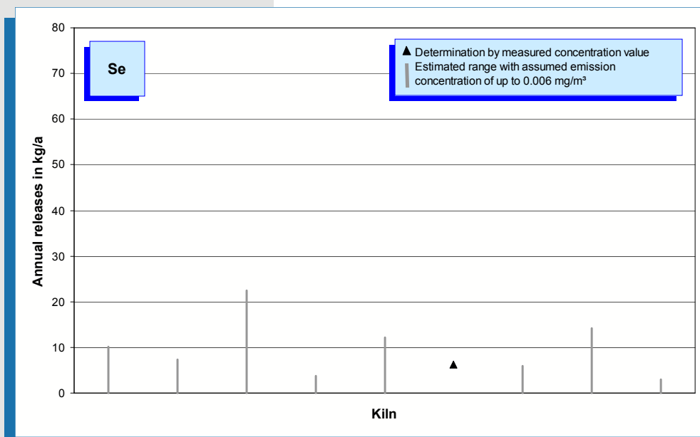
Fig. 5-54: Selenium emissions (annual releases in 2005) of nine rotary kilns.
