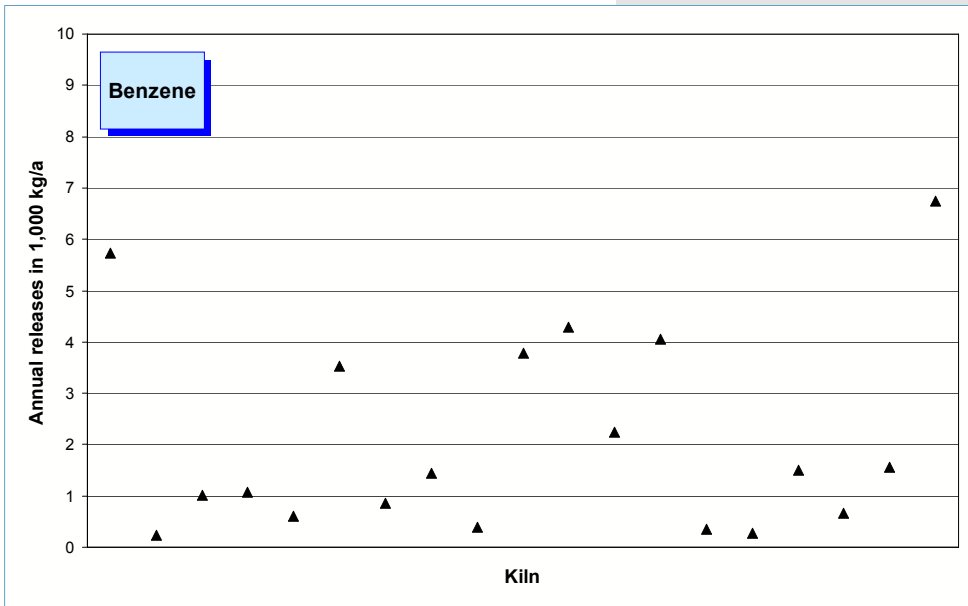
Fig. 5-20: Benzene emissions (annual releases in 2005) of 19 rotary kilns.
