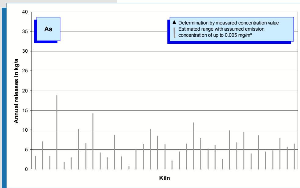
Fig. 5-34: Arsenic emissions (annual releases in 2005) of 37 rotary kilns.
