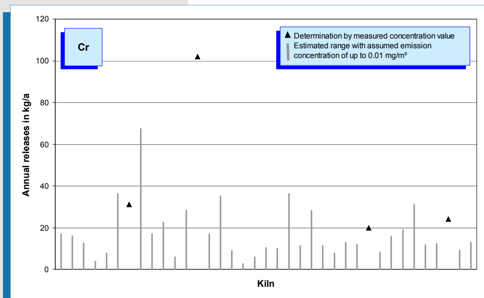
Fig. 5-38: Chromium emissions (annual releases in 2005) of 37 rotary kilns.
