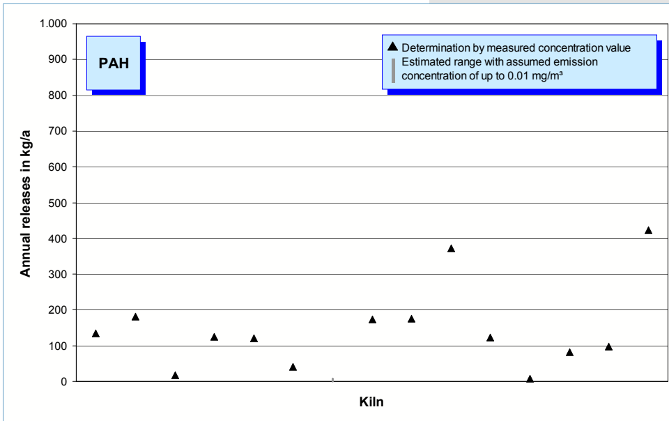
Fig. 5-16: PAH emissions (annual releases in 2005) of 15 rotary kilns.
