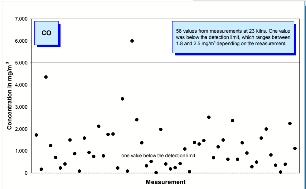
Fig. 5-7: CO concentration values (year 2005) measured in the clean gas of 23 rotary kilns.
