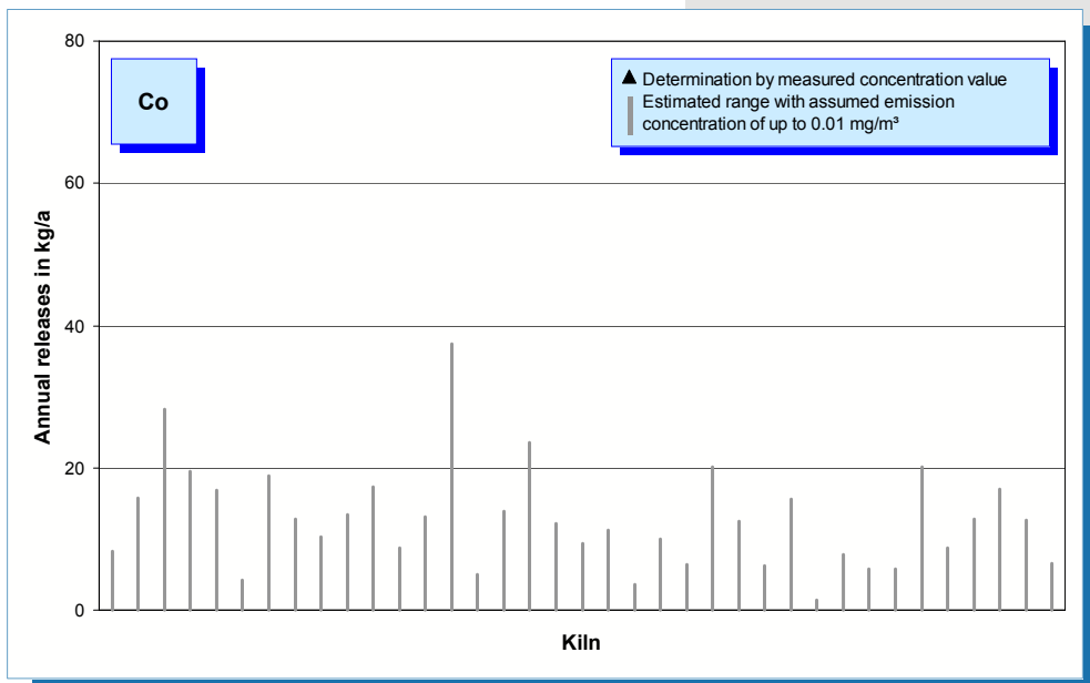
Fig. 5-40: Cobalt emissions (annual releases in 2005) of 37 rotary kilns.
