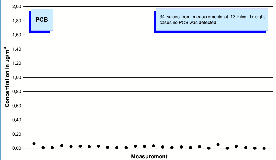
Fig. 5-13: Polychlorinated biphenyl (PCB according to DIN 51527) concentration values (year 2005) measured in the clean gas of 13 rotary kilns. In eight cases no PCB was detected. Note: there is no standardised test specification indicating the performance characteristics of the measuring method used for measuring PCB in the clean gas of rotary kilns. For that reason, no detection limit is given here. below 0.02 \mu\text{g}/\text{m}^3 the methods currently used do not provide secured emission concentrations.
