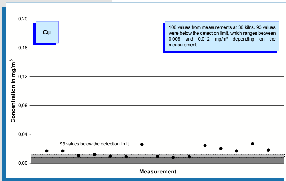
Fig. 5-41: Copper concentration values (year 2005) measured in the clean gas of 38 rotary kilns.
