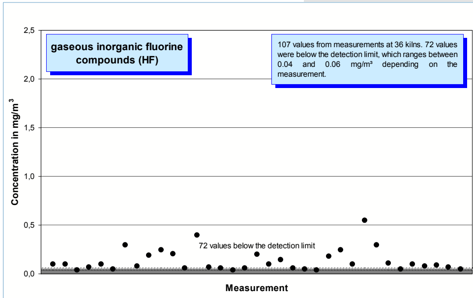
Fig. 5-23: Gaseous inorganic fluorine compound concentration values (year 2005) measured in the clean gas of 36 rotary kilns and given as HF.
