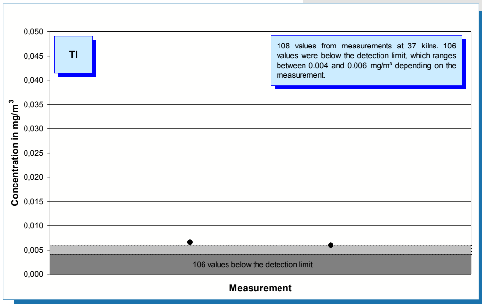
Fig. 5-27: Thallium concentration values (year 2005) measured in the clean gas of 37 rotary kilns.
