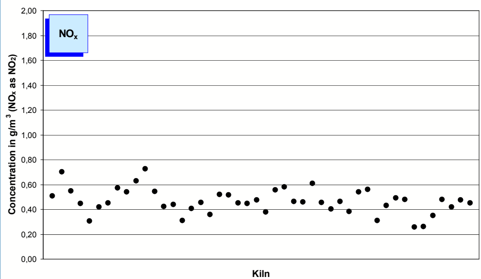
Fig. 5-3: Average NO x concentrations (year 2005) in the clean gas of 46 rotary kilns. Note: In 2005, the emissions of several kilns exceeded the emission values for cement plants specified by the Clean Air Act now. The operating permits for these works are based on higher NO x limits. Some of these plants have been shut down or will be shut down within the next few years, respectively, while others will be retrofitted with NO x reduction devices.
