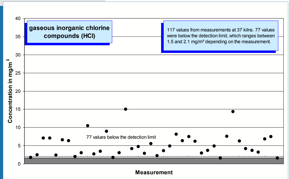
Fig. 5-21: Gaseous inorganic chlorine compound concentration values (year 2005) measured in the clean gas of 37 rotary kilns and given as HCl.
